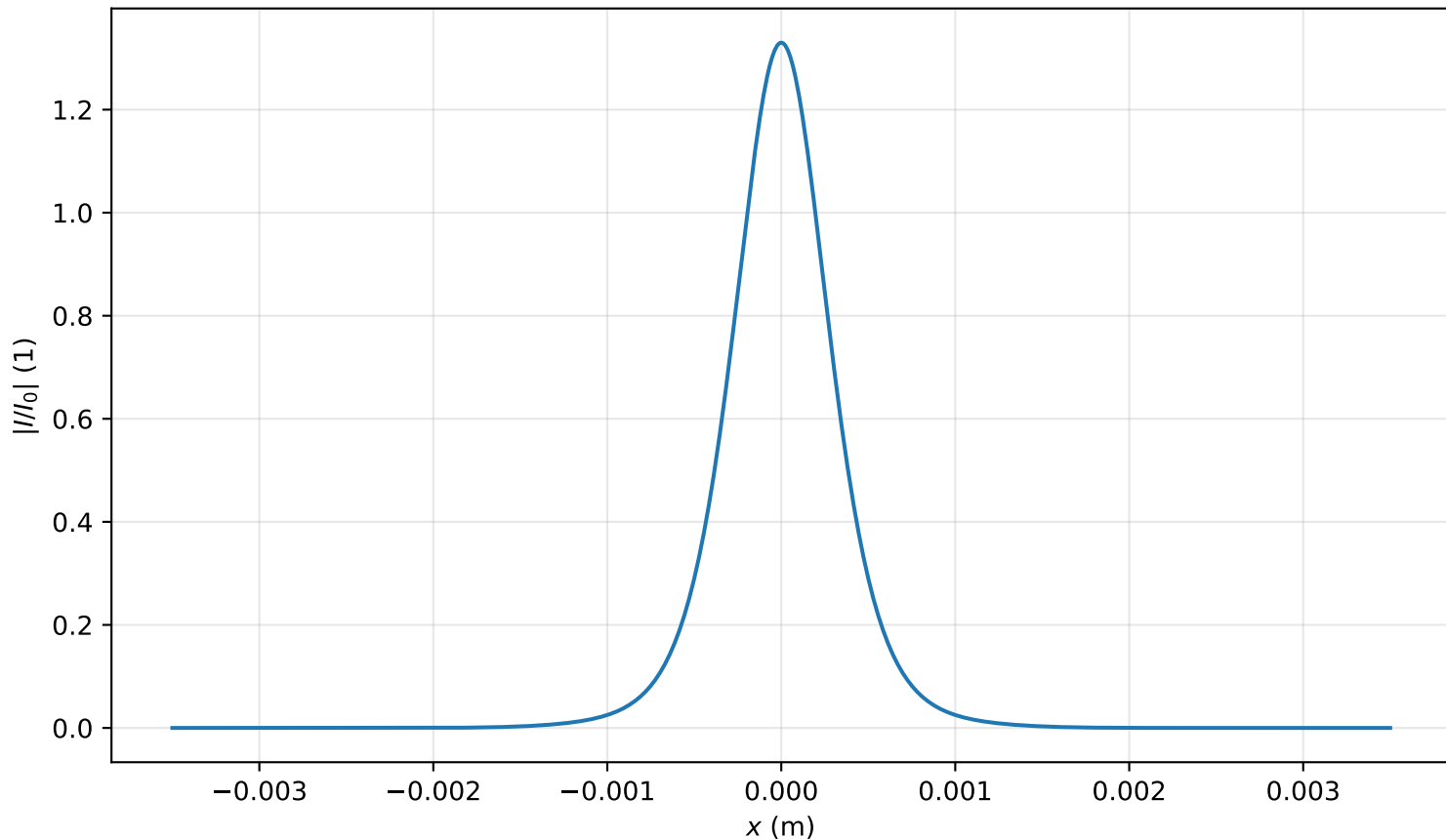
Intensity profile I(x, y = 0, z = 1.911m)/I_0 , P_{in}=0.8P_{cr} , artificial time
